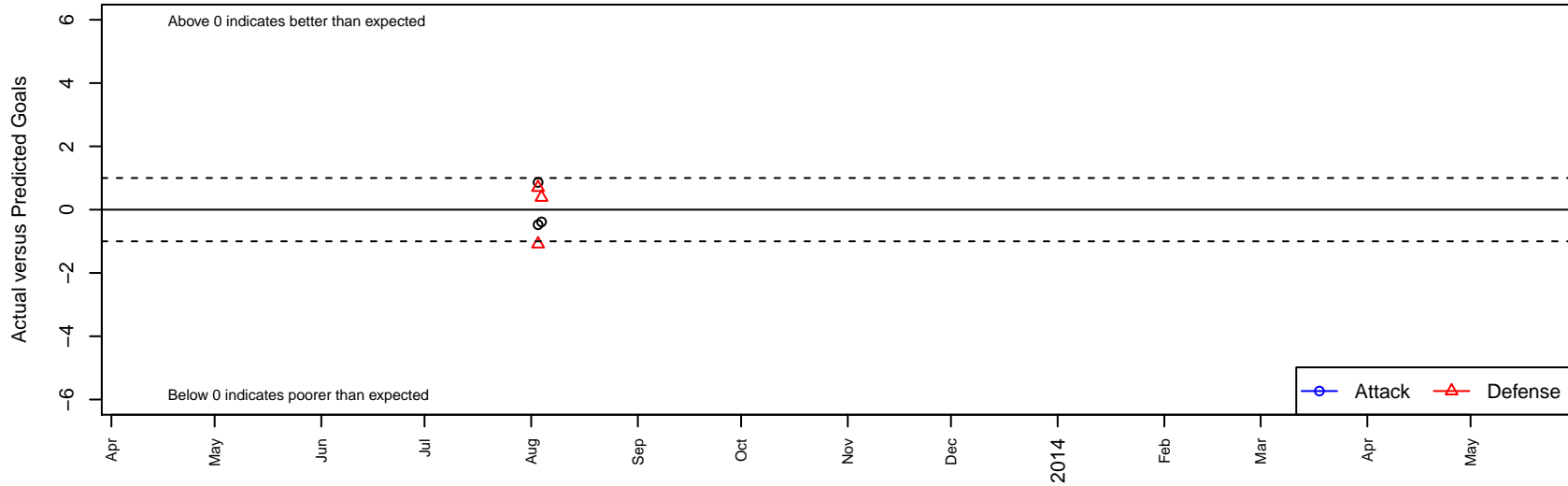
FC United Academy B01 Dots are actual minus expected GF (blue circles) and GA (red triangles). Blue line is smoothed change in attack strength. Red is smoothed change in defense strength.
